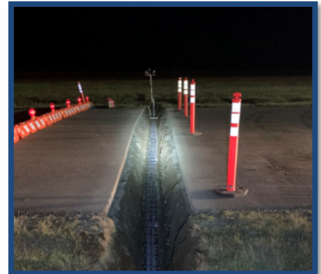
As seen in this night shift photo, rebar and new conduits installed across Taxiway Bravo prior to concrete pour.
